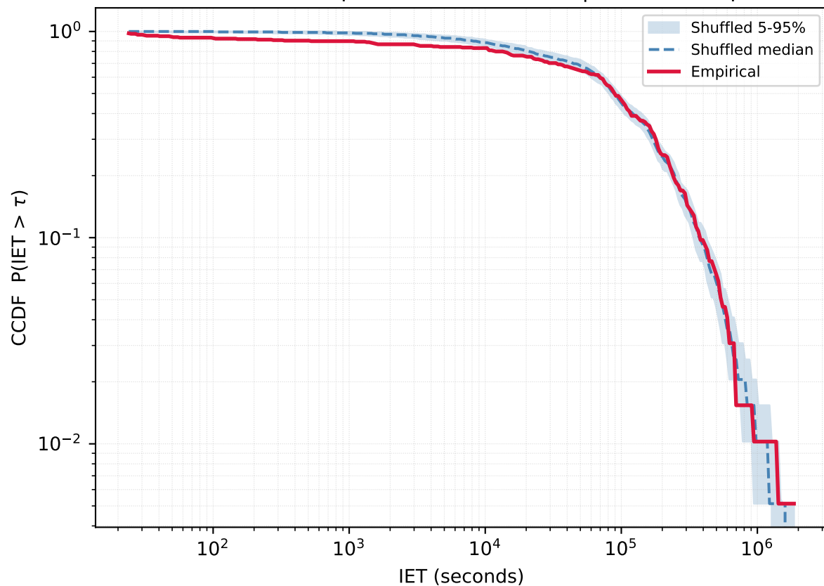
User 428716184 - Empirical vs Reshuffled | KS=0.109 p=0.030
